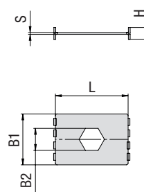
Safety Locking Plate SIV (Prevents Stacking Bolt from Loosening and Upper Clamp from Turning)
