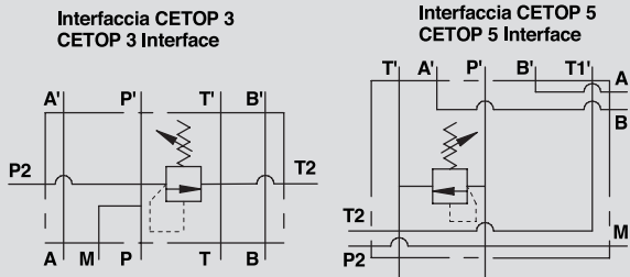
SCHEMA IDRAULICO HYDRAULIC DIAGRAM
