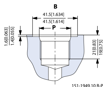
B: UNF Main port P: 1 \frac{1}{16} – 12 UN
