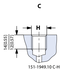
C: G Drain/release port H: ISO 228/1 – G \frac{1}{4}
