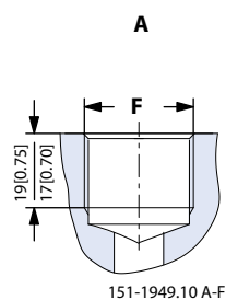
A: G Main port F: ISO 228/1 – G \frac{3}{4}
