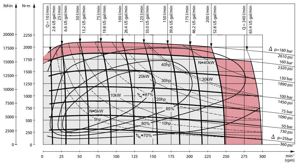
OMV 800 function diagram
