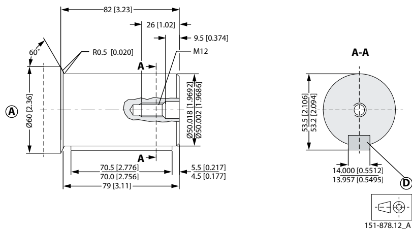
OMV shaft version
