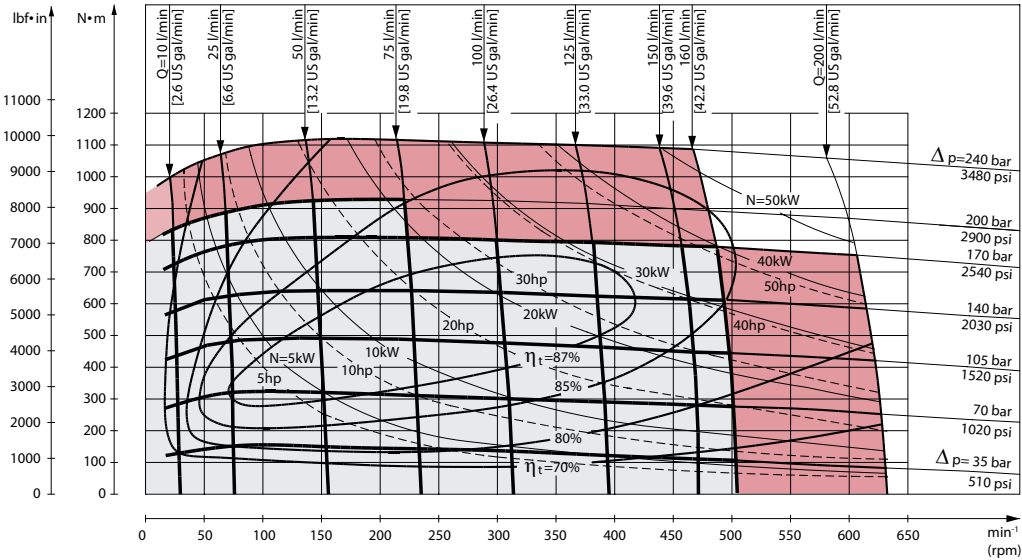
OMV 315 function diagram
