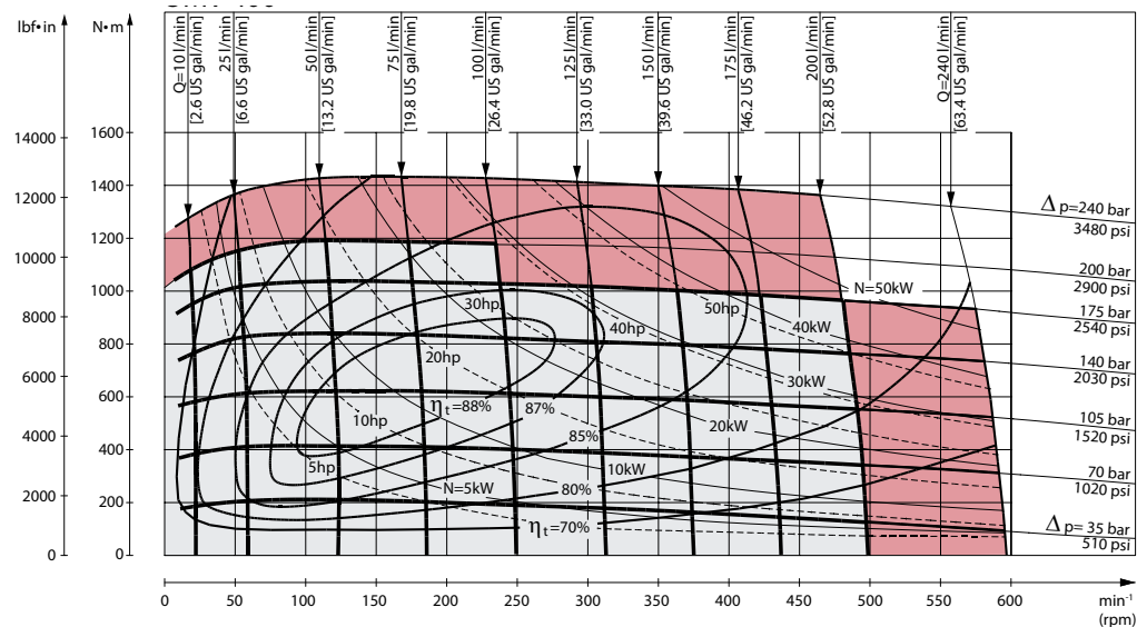
OMV 400 function diagram
