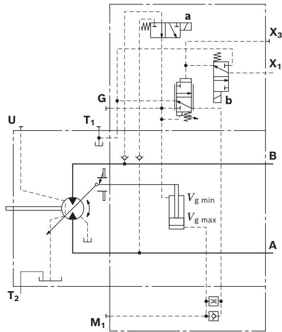
▼ Circuit diagram DA1, DA2 Size 28 to 215
